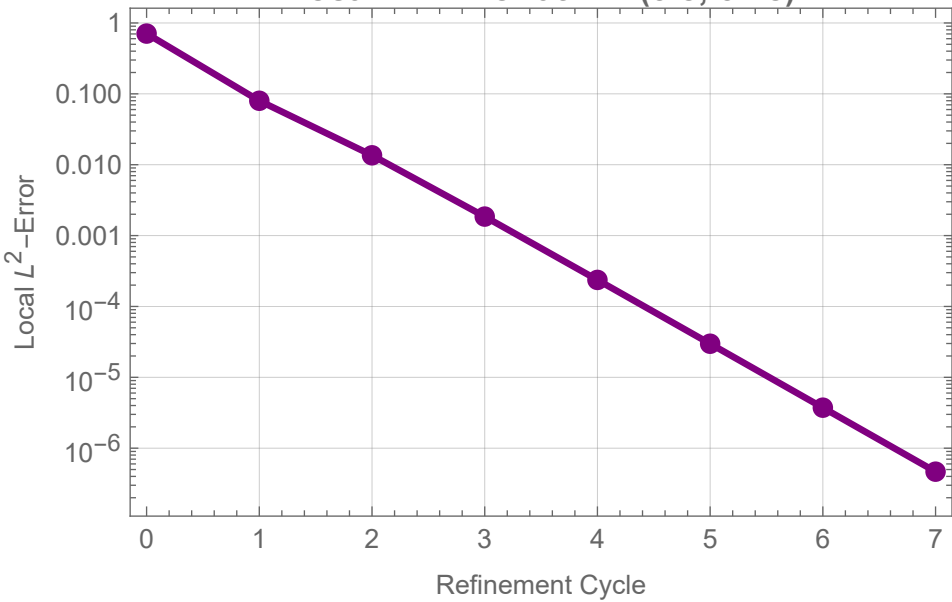
Local L^2 -Error at C = (0.5, 0.75)
